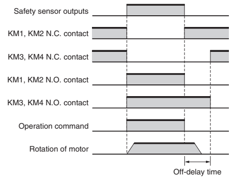
Timing chart
